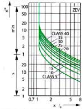
Tripping characteristics
